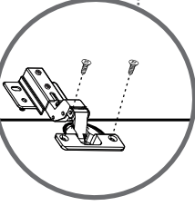
Bisagra Semi Parche/ Half Overlay Hinge
