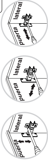
Bisagra Semi Parche/ Half Overlay Hinge
